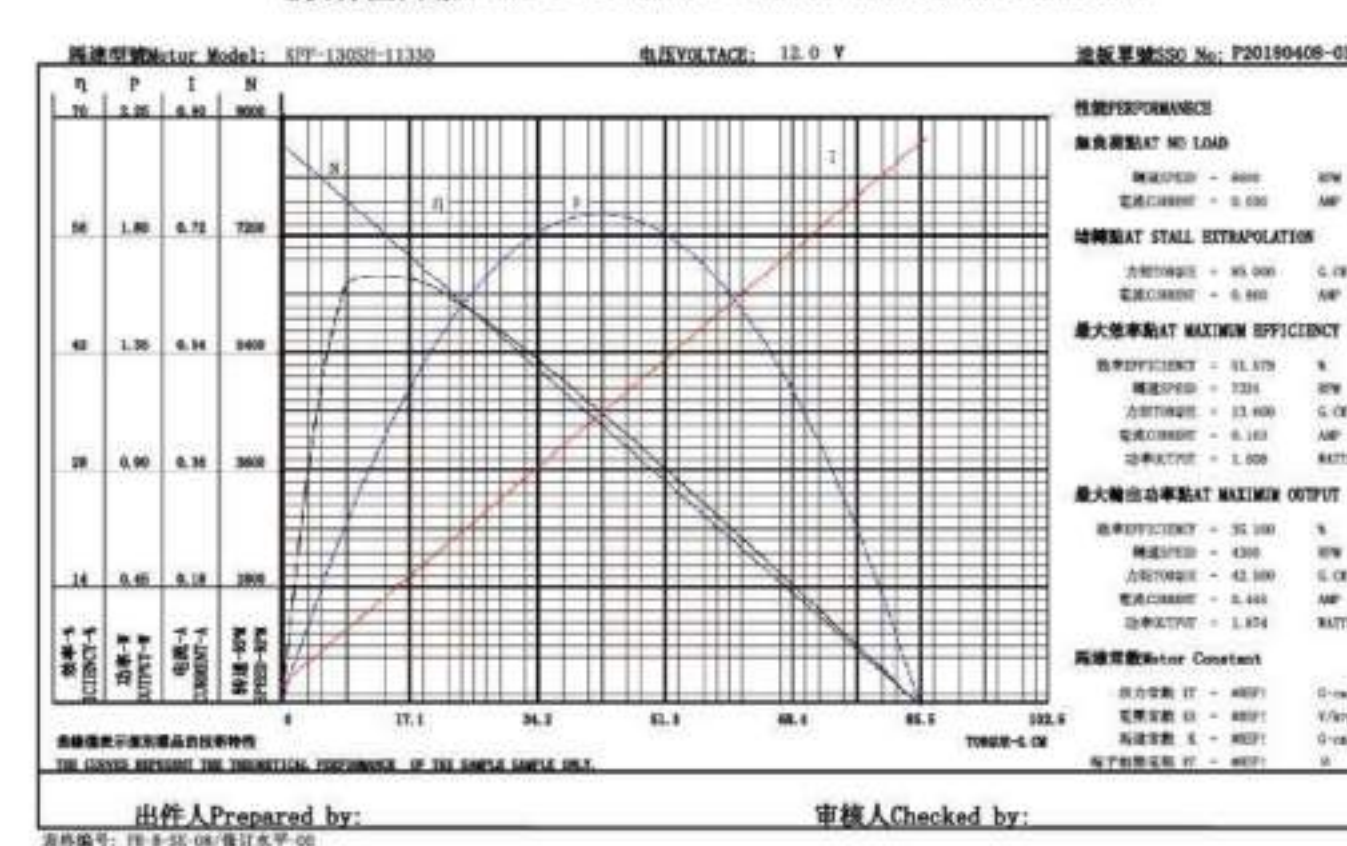
电机特性曲线 Motor Performance Curves and Characteristics
